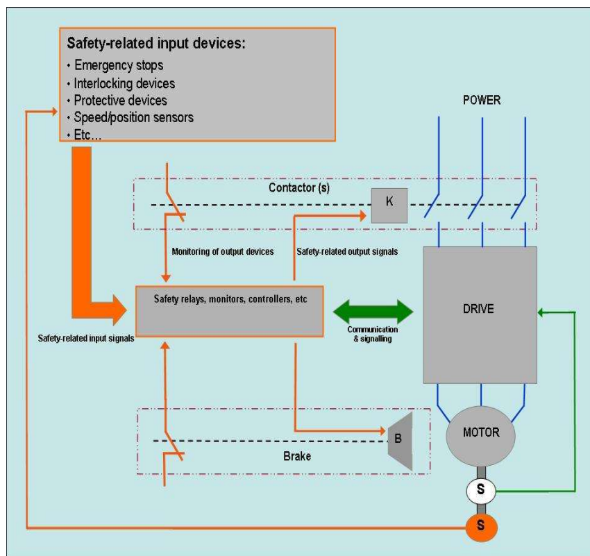
Figure 4 – Example of non safety-related drive supplemented by safety-related control measures
